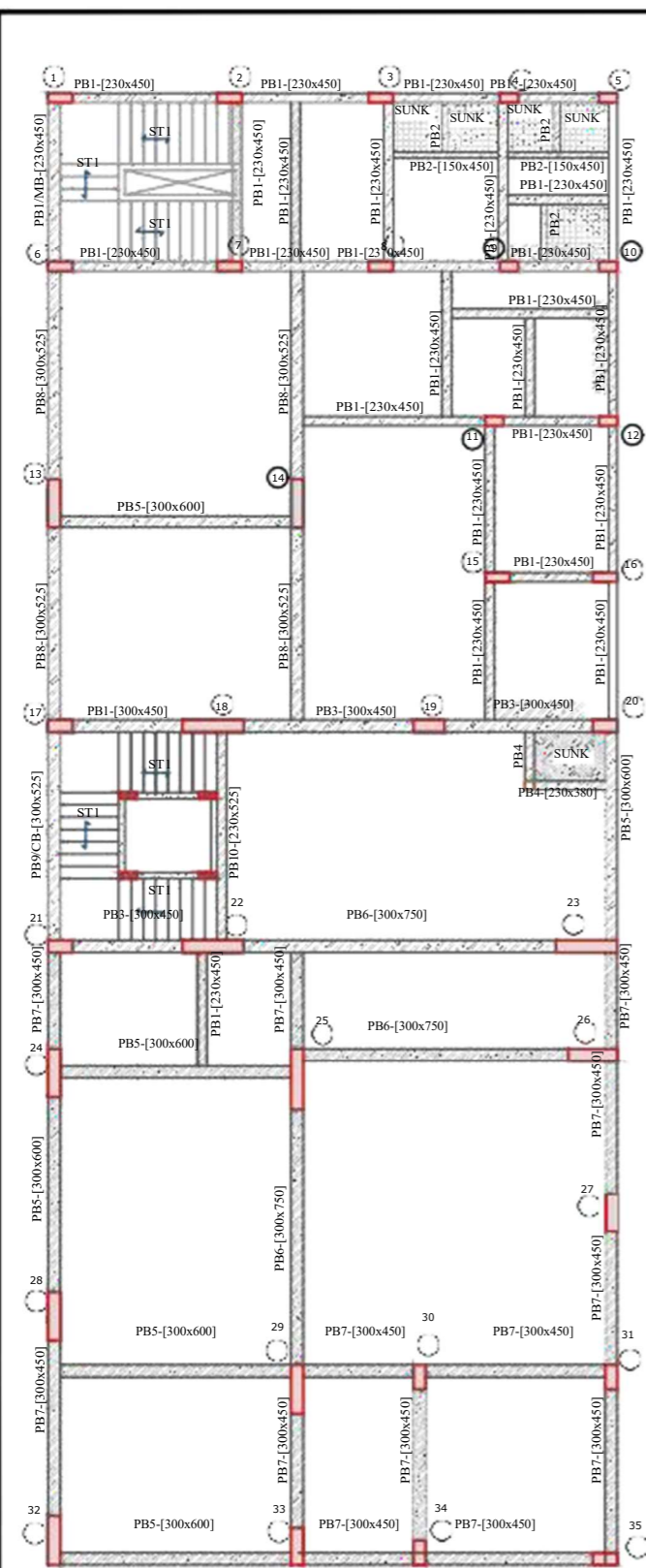
PLINTH BEAM FRAMING PLAN
