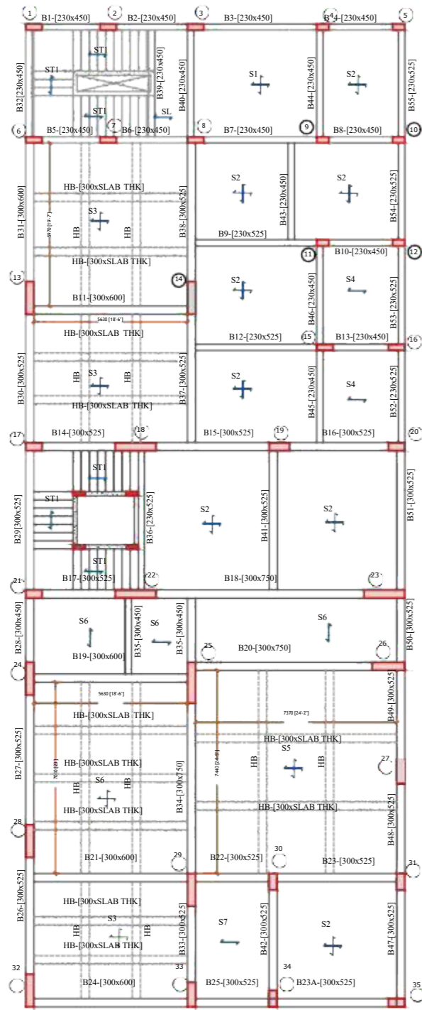
GROUND FLOOR SLAB & BEAM FRAMING PLAN
