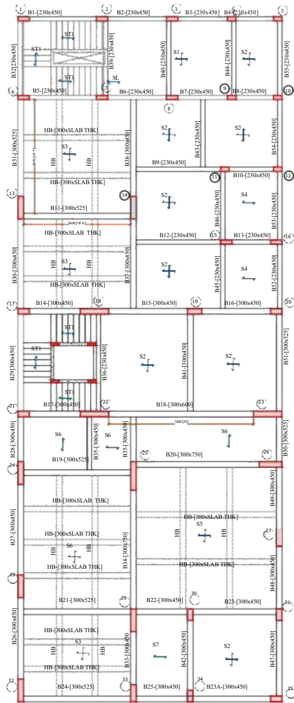
FIRST FLOOR SLAB & BEAM FRAMING PLAN
